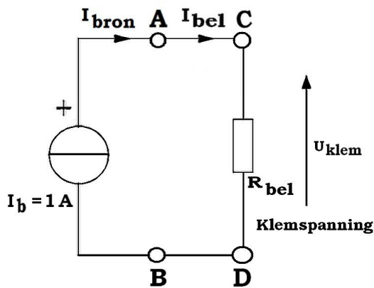
Ideale stroombron
